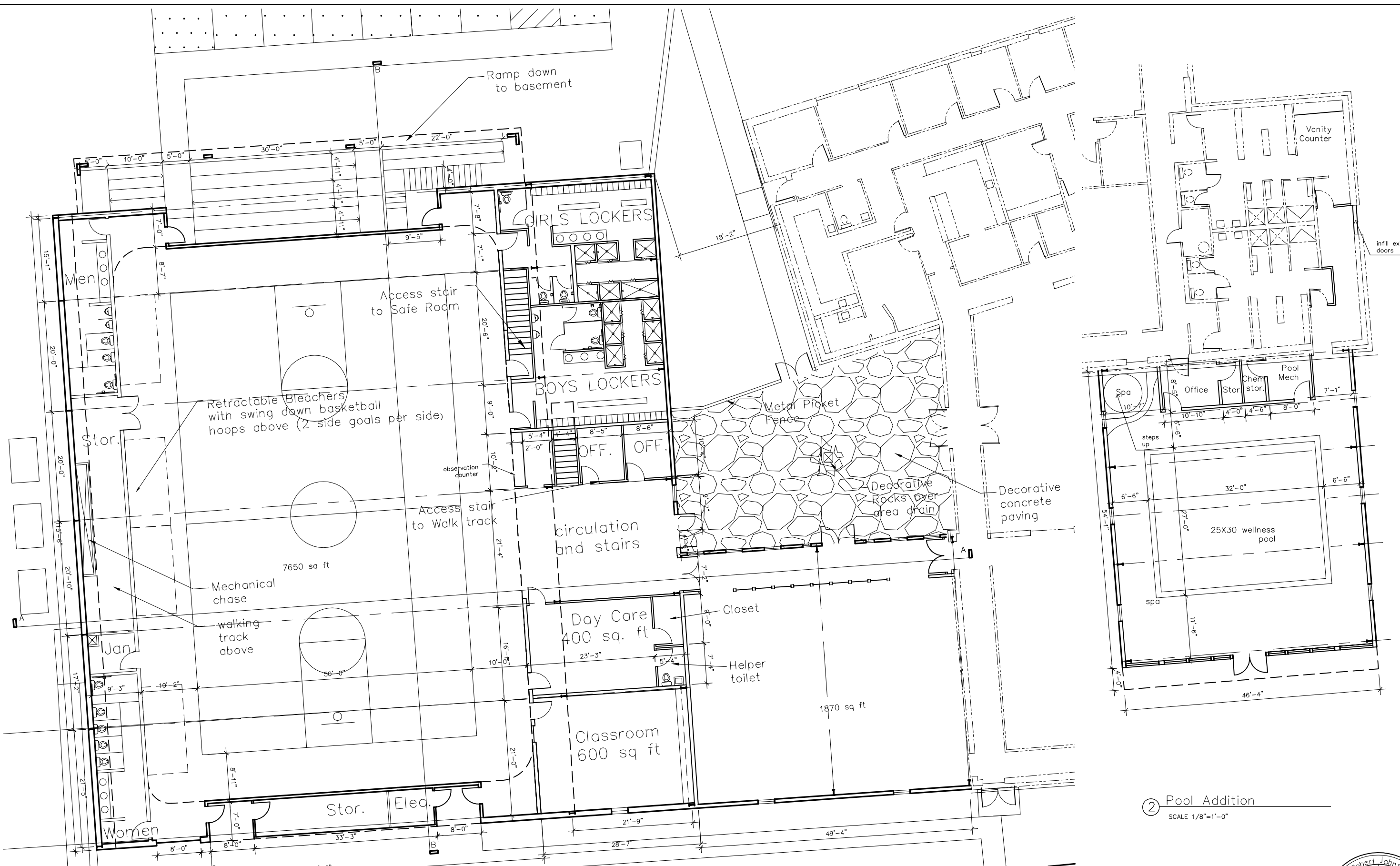
① Main Building SCALE 1/8"=1'-0"
